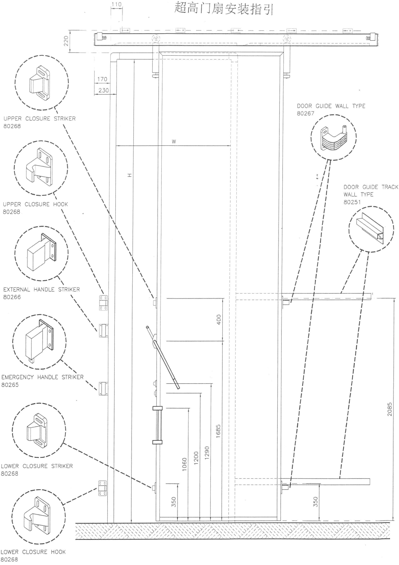
Door Leaf And Door Frame Installation Layout For Special Height 超高门扇及门洞安装指引
