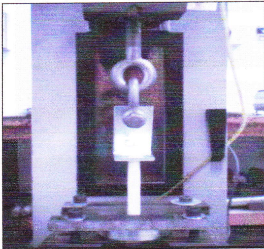
Photo 1.0 : Shows sample during test.
